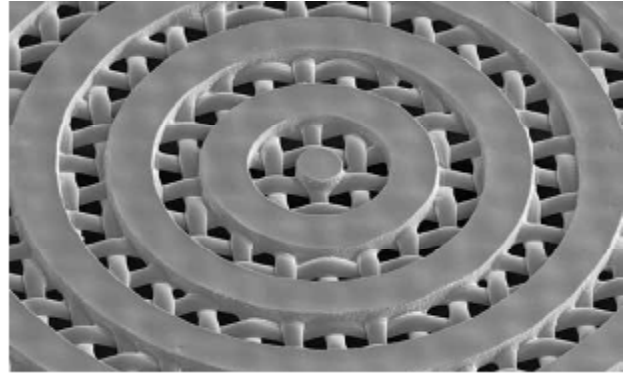
Sharp edged 80 µm circle line exposed on ARTLINE® PME 140/355-30Y
